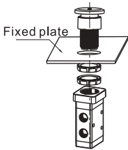
Fixation way of panel
